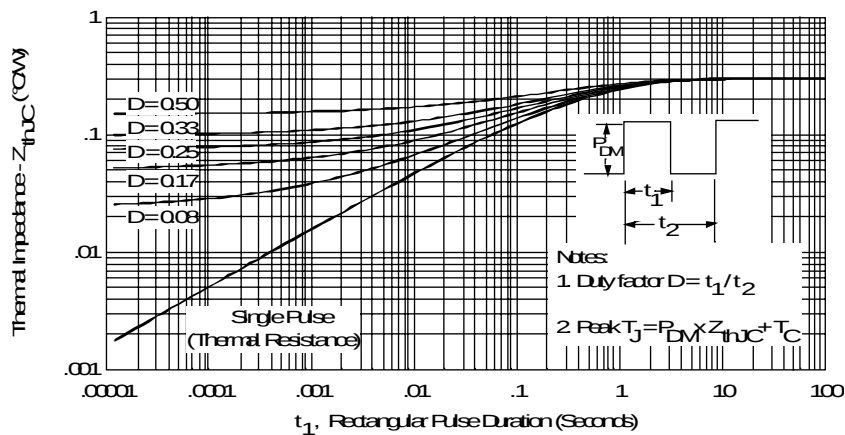
Fig. 4 - Maximum Thermal Impedance Z_{\theta JC} Characteristics
