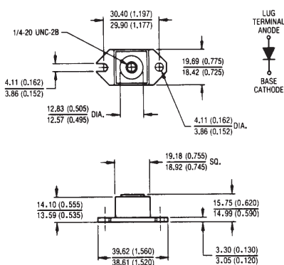
Outline HALF PAK Module Dimensions in millimeters and inches
