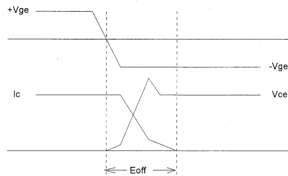
Turn-off Waveforms
