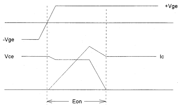
Turn-on Waveforms
