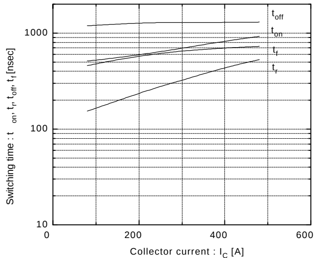
Switching time vs. Collector current V_{CC} = 600V, R_G = 2.7\Omega, V_{GE} = \pm 15V, T_J = 125^\circ\text{C}
