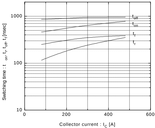
Switching time vs. Collector current V_{CC} = 600V, R_G = 2.7\Omega, V_{GE} = \pm 15V, T_J = 25^\circ\text{C}
