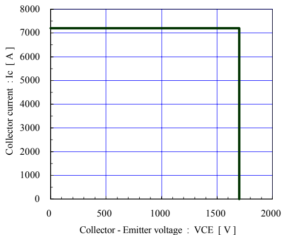
Reverse bias safe operating area (max.) \pm V_{GE}=15V , T_j=125^\circ C / chip
