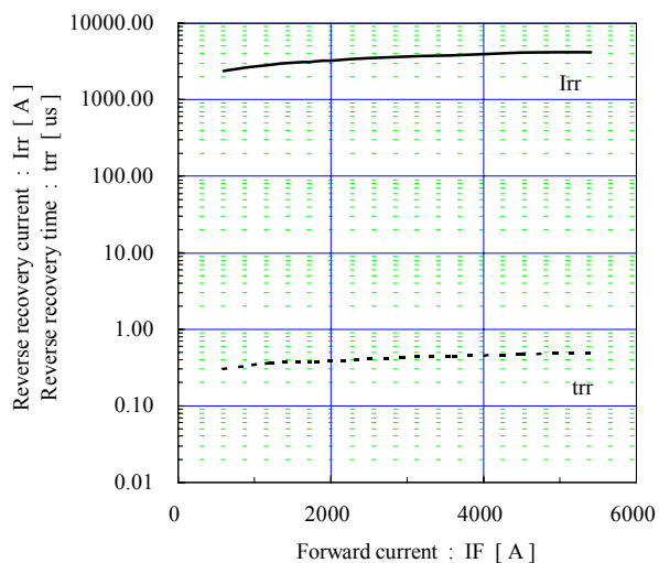
Reverse recovery characteristics (typ.) V_{cc}=900\text{V} , V_{GE}=\pm 15\text{V} , R_g=0.1\Omega , T_j=125^{\circ}\text{C}
