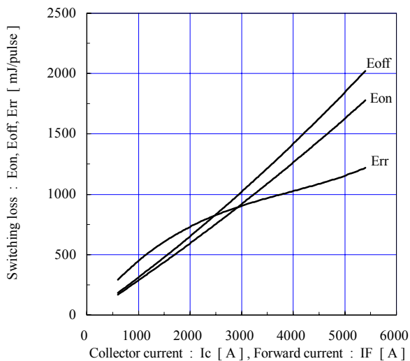
Switching loss vs. Collector current (typ.) V_{cc}=900V , V_{GE}=\pm 15V , R_{gon}=0.1\Omega , R_{goff}=0.2\Omega , T_j=125^\circ C
