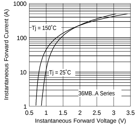
Fig. 7 - Forward Voltage Drop Characteristics Maximum Allowable Ambient T_a
