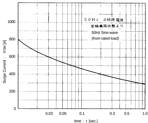
Surge Current
