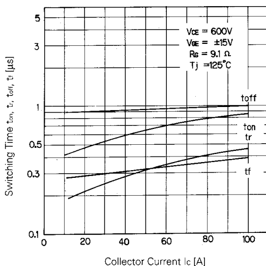
Switching Time
