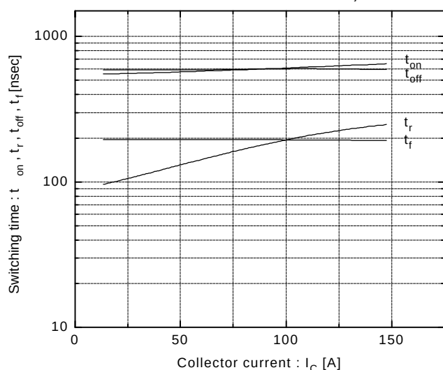
Switching time vs. Collector current V_{CC} = 300V, R_G = 24\Omega, V_{GE} = \pm 15V, T_j = 25^\circ\text{C}
