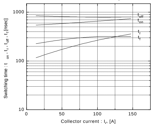
Switching time vs. Collector current V_{CC} = 300V, R_G = 24\Omega, V_{GE} = \pm 15V, T_j = 125^\circ\text{C}
