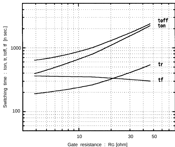
Switching time vs. R_G V_{CC}=600V , I_C=100A , V_{GE}=\pm 15V , T_J=25^\circ C
