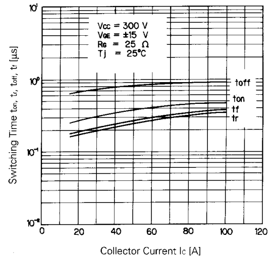
Switching Time
