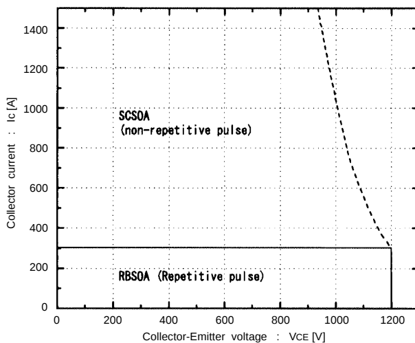
Reversed biased safe operating area +V_{GE}=15V , -V_{GE} \leq 15V , T_J \leq 125^\circ C , R_G \geq 5.6\text{ ohm}
