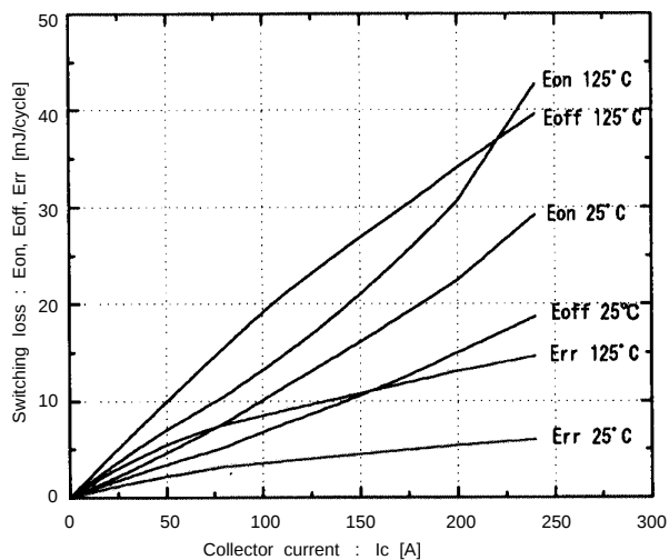
Switching loss vs. Collector current V_{CC}=600V , R_G=5.6\text{ ohm} , V_{GE}=\pm 15V
