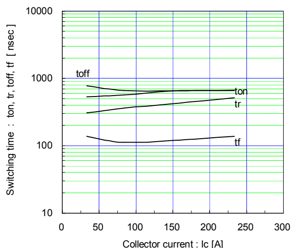
Switching time vs. Collector current (typ.) Vcc=900V, VGE=±15V, Rg=3.3Ω, Tj=125°C
