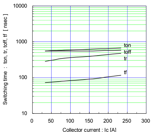
Switching time vs. Collector current (typ.) Vcc=900V, VGE=±15V, Rg=3.3Ω, Tj= 25°C
