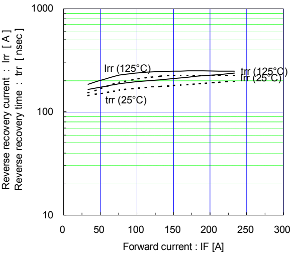
Reverse recovery characteristics (typ.) Vcc=900V, VGE=±15V, Rg=3.3Ω
