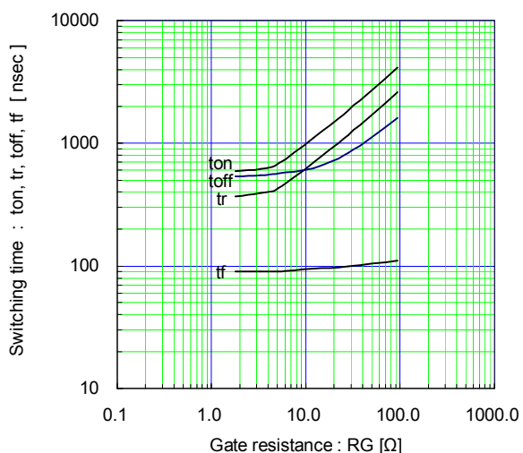
Switching time vs. Gate resistance (typ.) Vcc=900V, Ic=150A, VGE=±15V, Tj= 25°C
