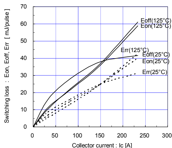
Switching loss vs. Collector current (typ.) Vcc=900V, VGE=±15V, Rg=3.3Ω
