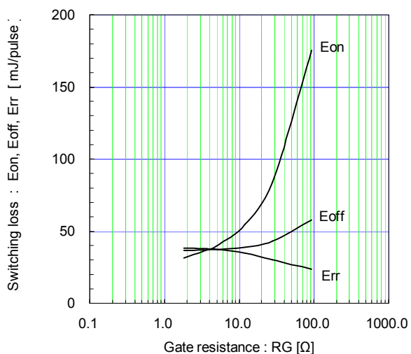
Switching loss vs. Gate resistance (typ.) Vcc=900V, Ic=150A, VGE=±15V, Tj= 125°C
