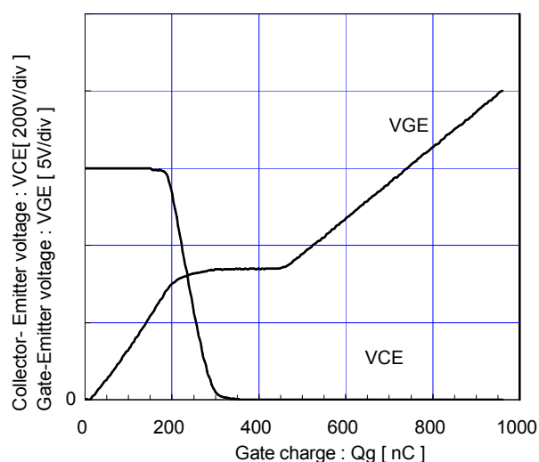
Dynamic Gate charge (typ.) Vcc=600V, Ic=200A, Tj=25°C
