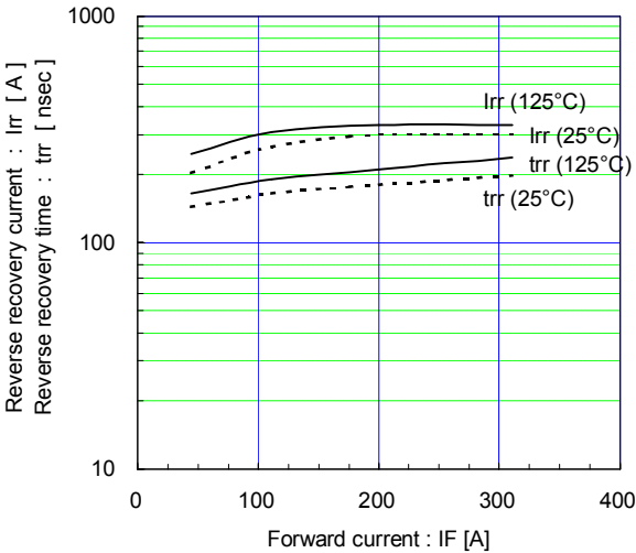
Reverse recovery characteristics (typ.) Vcc=900V, VGE=±15V, Rg=2.2Ω
