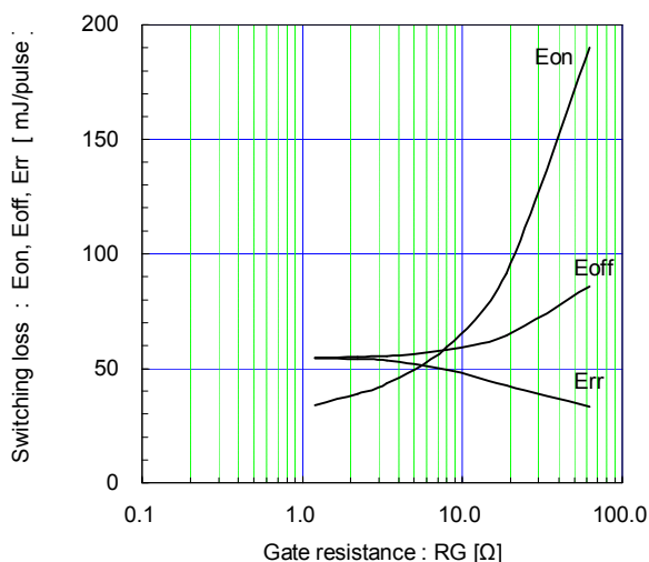
Switching loss vs. Gate resistance (typ.) V_{CC}=900V , I_c=200A , V_{GE}=\pm 15V , T_j=125^\circ C
