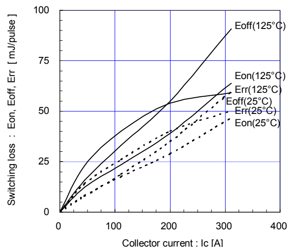
Switching loss vs. Collector current (typ.) V_{CC}=900V , V_{GE}=\pm 15V , R_g=2.2\Omega
