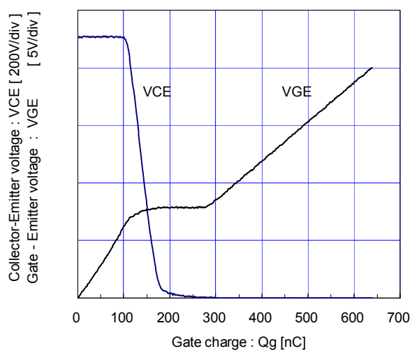
Dynamic Gate charge (typ.) Vcc=900V, Ic=200A, Tj= 25°C
