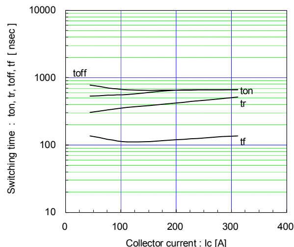
Switching time vs. Collector current (typ.) V_{CC}=900V , V_{GE}=\pm 15V , R_g=2.2\Omega , T_j=125^\circ C
