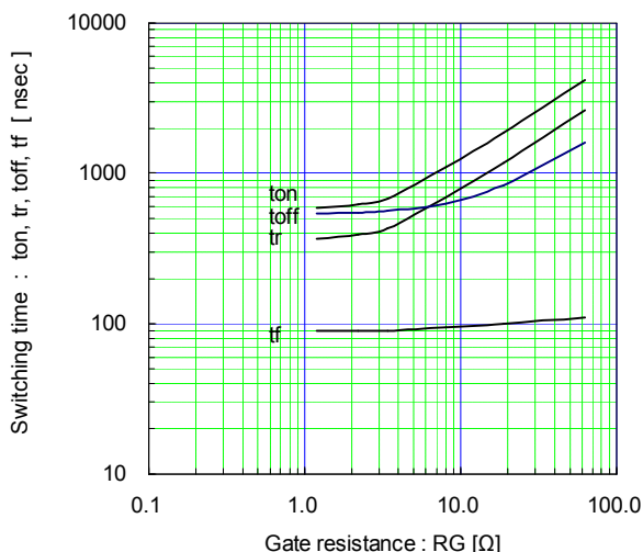
Switching time vs. Gate resistance (typ.) V_{CC}=900V , I_c=200A , V_{GE}=\pm 15V , T_j=25^\circ C
