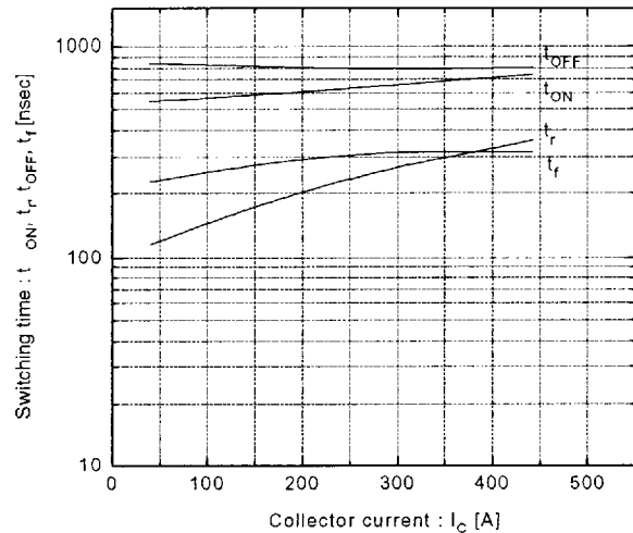
Switching time vs. Collector current V_{CC} = 300\text{V} , R_G = 6.8\Omega , V_{GE} = \pm 15\text{V} , T_J = 125^\circ\text{C}
