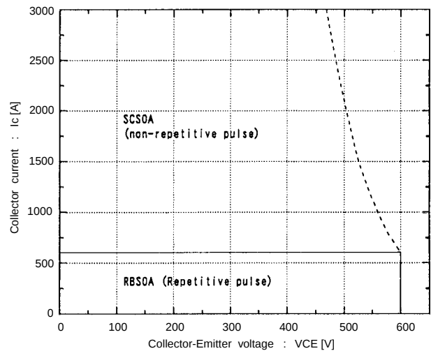
Reversed biased safe operating area +V_{GE}=15V , -V_{GE} \leq 15V , T_J \leq 125^\circ C , R_G \geq 6.8\Omega
