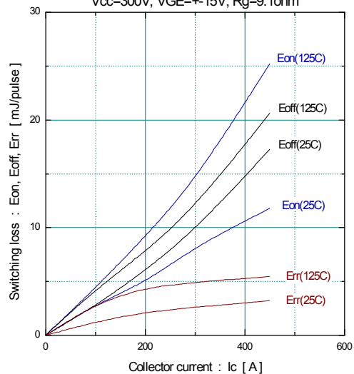
[ Inverter ] Switching loss vs. Collector current (typ.) V_{cc}=300V , V_{GE}=\pm 15V , R_g=9.1\Omega
