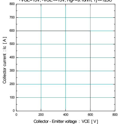
[ Inverter ] Reverse bias safe operating area +V_{GE}=15V , -V_{GE}\leq 15V , R_g\geq 9.1\Omega , T_j\leq 125^\circ C
