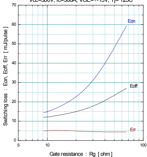
[ Inverter ] Switching loss vs. Gate resistance (typ.) V_{cc}=300V , I_c=300A , V_{GE}=\pm 15V , T_j=125^\circ C
