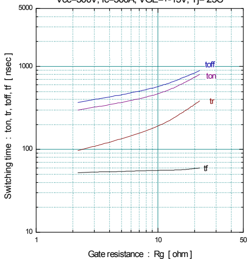
[ Inverter ] Switching time vs. Gate resistance (typ.) V_{cc}=300V , I_c=300A , V_{GE}=\pm 15V , T_j=25^\circ C
