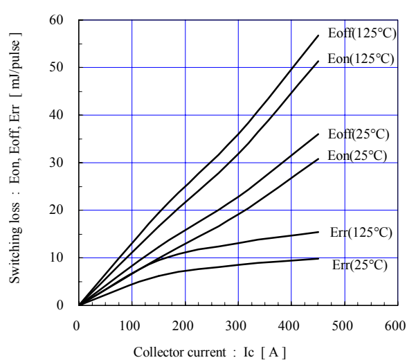
Switching loss vs. Collector current (typ.) V_{cc}=600V , V_{GE}=\pm 15V , R_g=1.1\Omega
