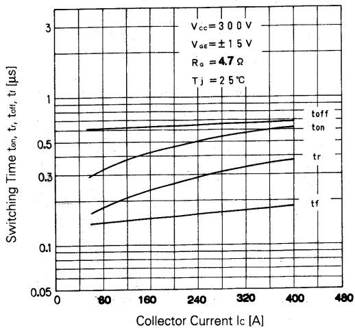
Switching Time
