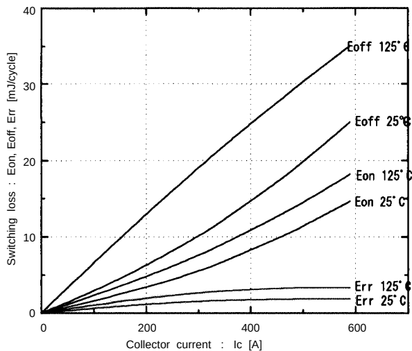
Switching loss vs. Collector current V_{CC}=300V , R_G=4.7 ohm, V_{GE}=\pm 15V
