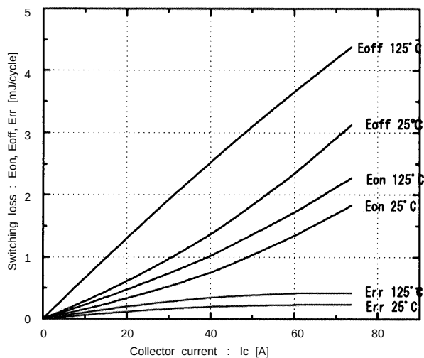
Switching loss vs. Collector current V_{CC}=300V , R_G=51\text{ ohm} , V_{GE}=\pm 15V
