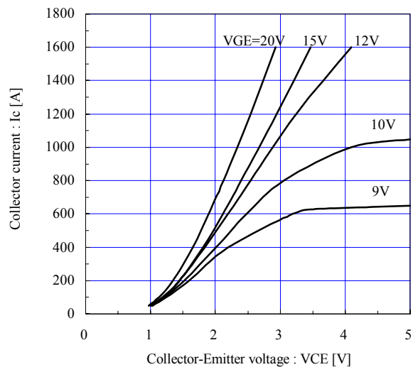
Collector current vs. Collector-Emitter voltage (typ.) Tj= 125°C, sense terminal
