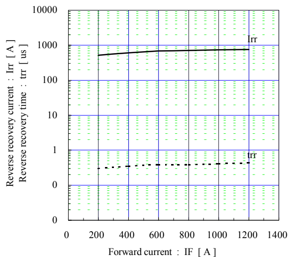
Reverse recovery characteristics (typ.) V_{cc}=900\text{V} , V_{GE}=\pm 15\text{V} , R_g=1.0\Omega , T_j=125^{\circ}\text{C}
