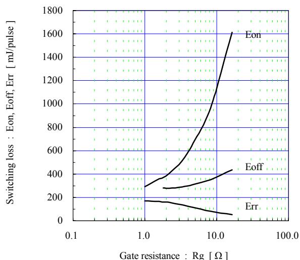
Switching loss vs. Gate resistance (typ.) V_{cc}=900V , I_c=800A , V_{GE}=\pm 15V , T_j=125^\circ C
