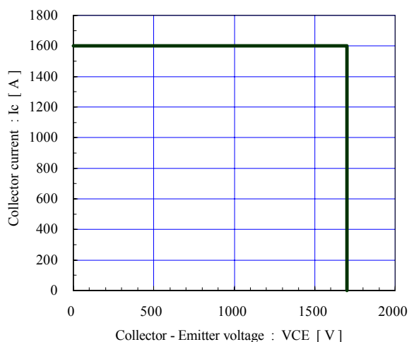
Reverse bias safe operating area (max.) \pm V_{GE}=15V , R_{goff}=1.8\Omega , T_j=125^\circ C / chip
