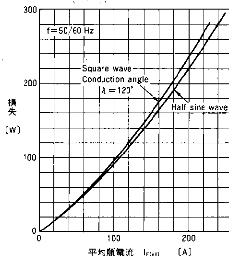
総損失—出力電流 Power Loss—Output Current
