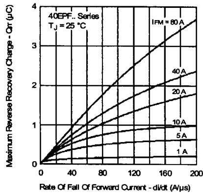
Fig. 10 - Recovery Charge Characteristics, T_j = 25^\circ\text{C}
