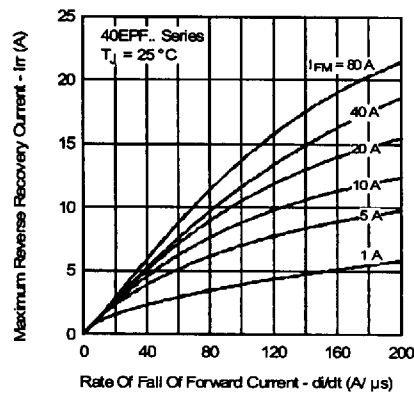
Fig. 12 - Recovery Current Characteristics, T_j = 25^\circ\text{C}
