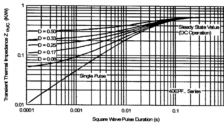
Fig. 14 - Thermal Impedance Z_{thJC} Characteristics
