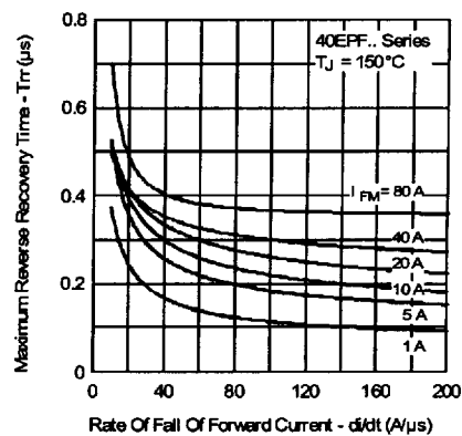
Fig. 9 - Recovery Time Characteristics, T_J = 150^\circ\text{C}
