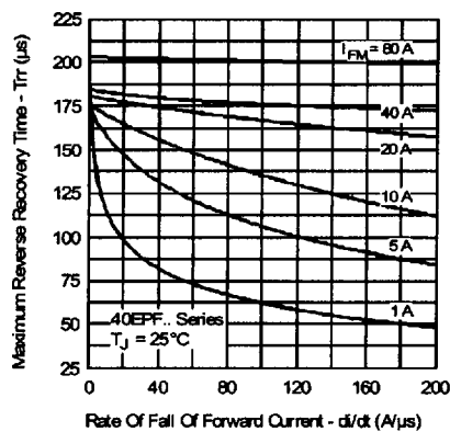
Fig. 8 - Recovery Time Characteristics, T_J = 25^\circ\text{C}
