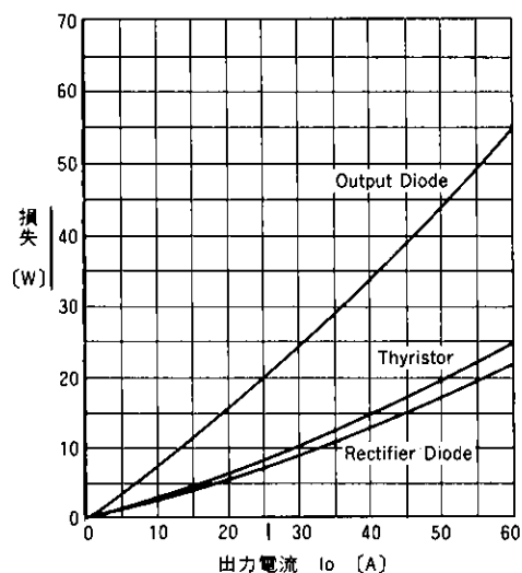
損失—出力電流(1素子あたり) Power Loss vs. Output Current (Per 1 chip)
