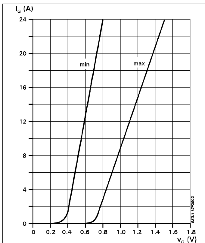
Fig. 7 Forward gate current vs. forward gate voltage.
