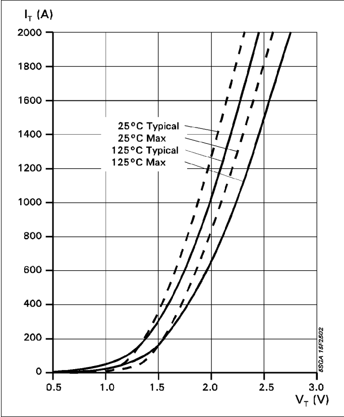
Fig. 2 On-state characteristics
