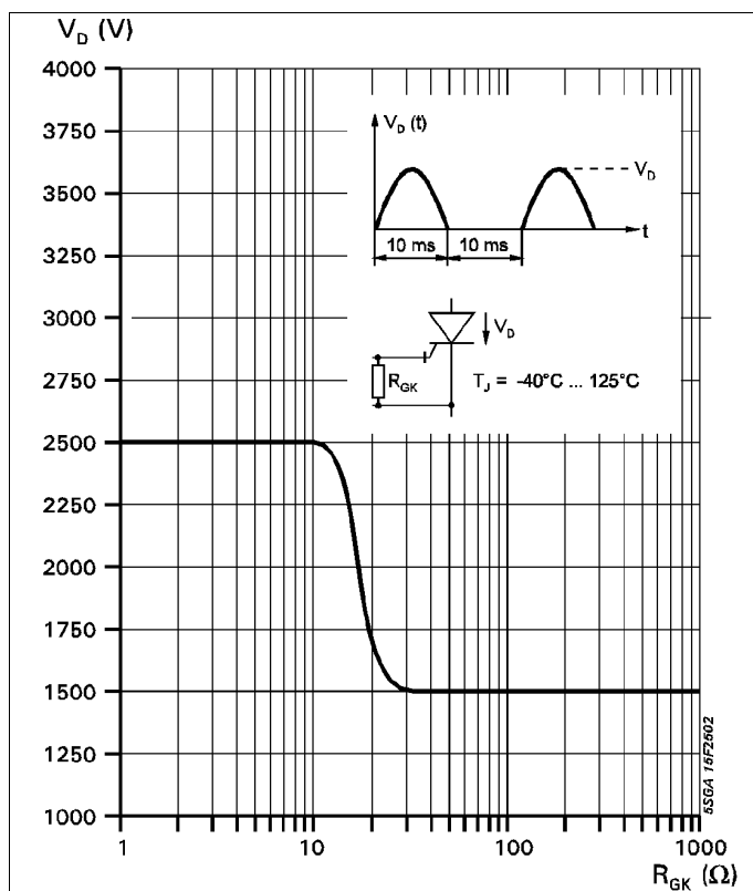
Fig. 5 Forward blocking voltage vs. gate-cathode resistance.
