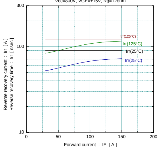
Reverse recovery characteristics (typ.) V_{CC}=800\text{V} , V_{GE}=\pm 15\text{V} , R_g=120\Omega
