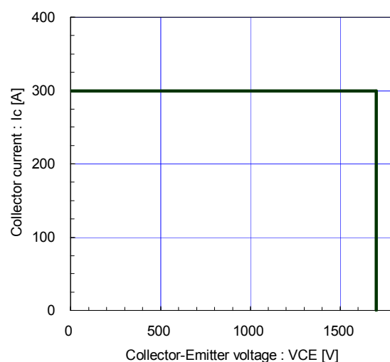
Reverse bias safe operating area (max.) +V_{GE}=15V , -V_{GE} \leq 15V , R_g \geq 3.3\Omega , T_j \leq 125^\circ C
