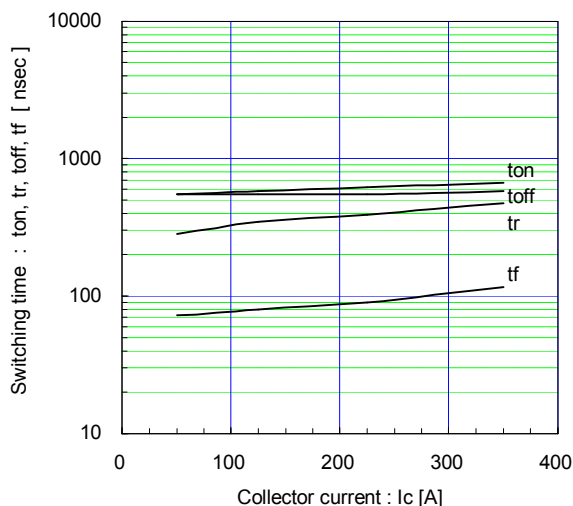
Switching time vs. Collector current (typ.) V_{CC}=900V , V_{GE}=\pm 15V , R_g=2.2\Omega , T_j=25^\circ C
