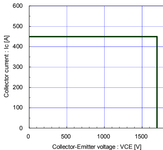
Reverse bias safe operating area (max.) +V_{GE}=15V , -V_{GE} \leq 15V , R_g \geq 2.2\Omega , T_j \leq 125^\circ C Stray inductance \leq 100nH
