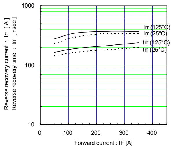
Reverse recovery characteristics (typ.) V_{cc}=900V , V_{GE}=\pm 15V , R_g=2.2\Omega
