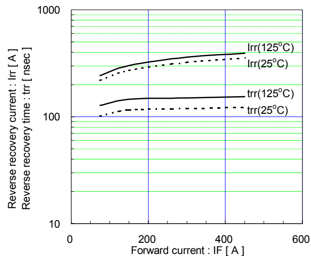
Reverse recovery characteristics (typ.) V_{CC}=600\text{V} , V_{GE}=\pm 15\text{V} , R_G=2.0\Omega
