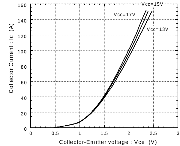
Collector current vs. Collector-Emittter voltage Tj=25°C
