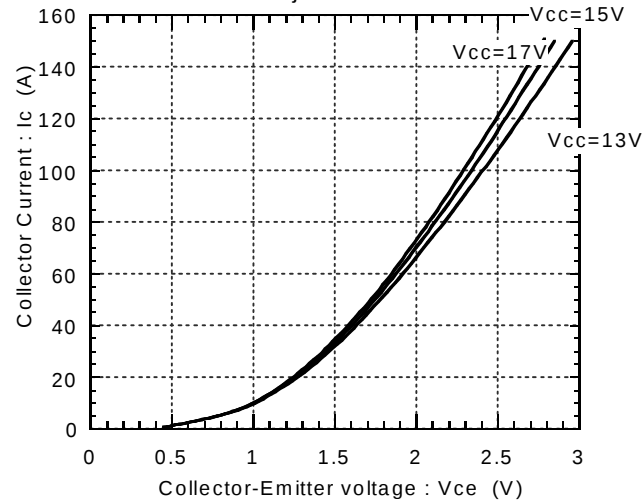
Collector current vs. Collector-Emittter voltage Tj=125°C
