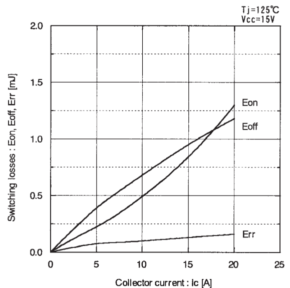
Switching losses vs. Collector current
