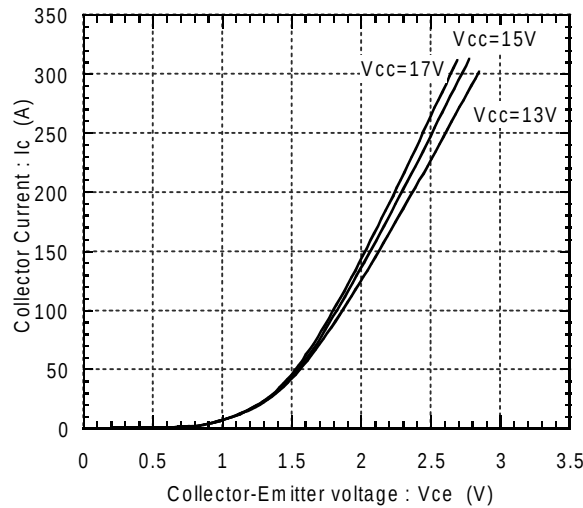
Collector current vs. Collector-Emmitter voltage T_j=25^{\circ}\text{C}
