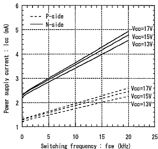
Power supply current vs. Switching frequency T_c=25^\circ\text{C}
