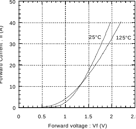
Forward current vs. Forward voltage (typ.) Terminal
