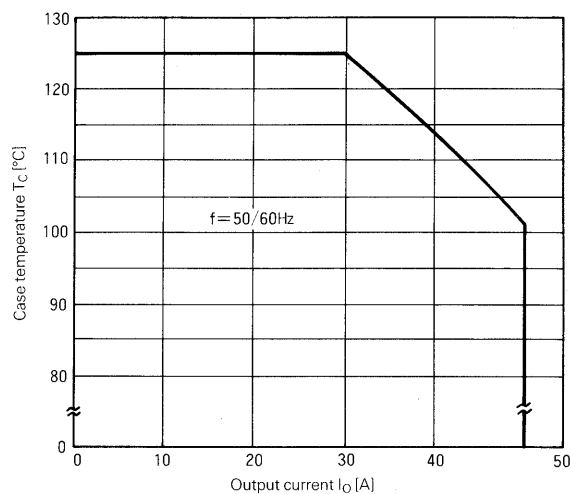
Case Temperature-Output Current
