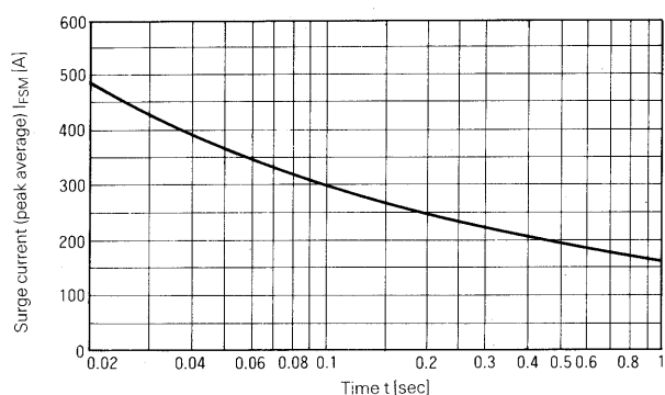
Surge Current
