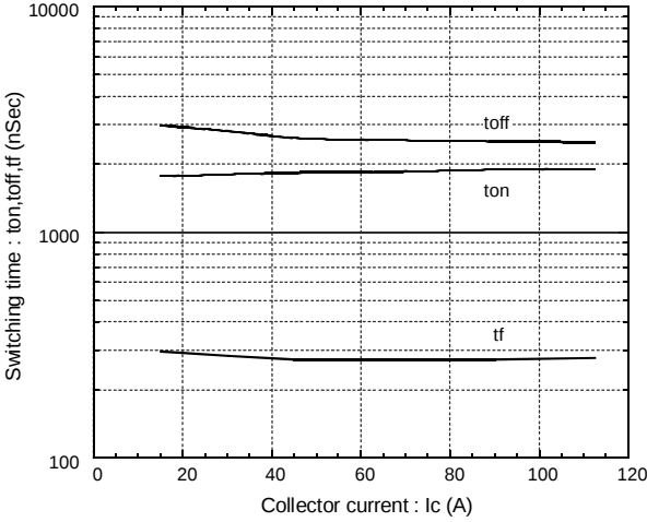
Switching time vs. Collector current Edc=600V,Vcc=15V,Tj=125°C
