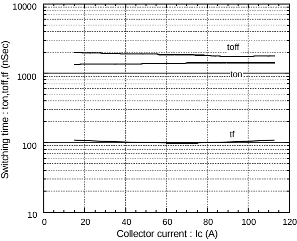
Switching time vs. Collector current Edc=600V,Vcc=15V,Tj=25°C
