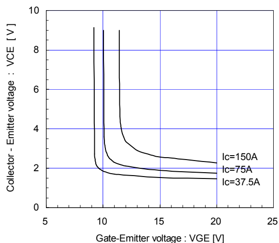
[ Inverter ] Collector-Emitter voltage vs. Gate-Emmitter voltage (typ.) T_j = 25^\circ\text{C} / chip
