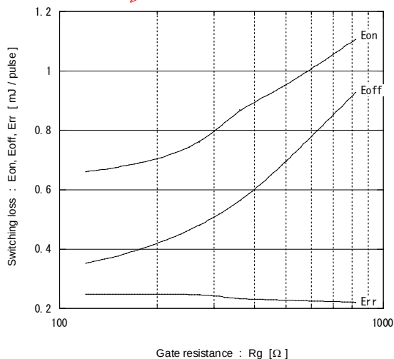
[ Inverter ] Switching loss vs. Gate resistance (typ.) V_{CC}=300V , I_c=15A , V_{GE}=+15V , T_j=125^\circ C
