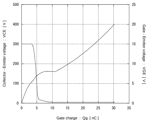
[ Brake ] Dynamic Gate charge (typ.) V_{CC} = 300\text{V}, I_C = 4\text{A}, T_J = 25^\circ\text{C}
