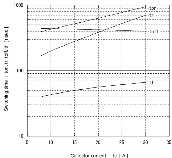
[ Inverter ] Switching time vs. Collector current (typ.) V_{CC}=300V , V_{GE}=+15V , R_g=270\Omega , T_j=125^\circ C
