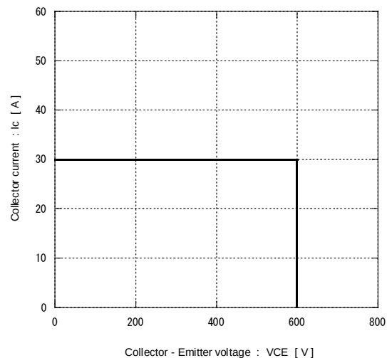
[ Inverter ] Reverse bias safe operating area +V_{GE}=15V , -V_{GE}\leq 15V , R_g\geq 270\Omega , T_j\leq 125^\circ C
