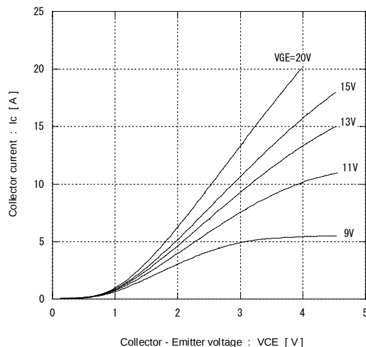
[ Brake ] Collector current vs. Collector-Emitter voltage T_J = 125^\circ\text{C}(\text{typ.}) / \text{chip}
