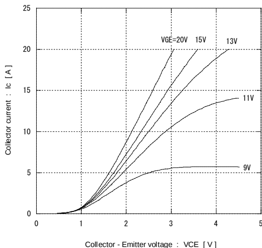
[ Brake ] Collector current vs. Collector-Emitter voltage T_J = 25^\circ\text{C}(\text{typ.}) / \text{chip}
