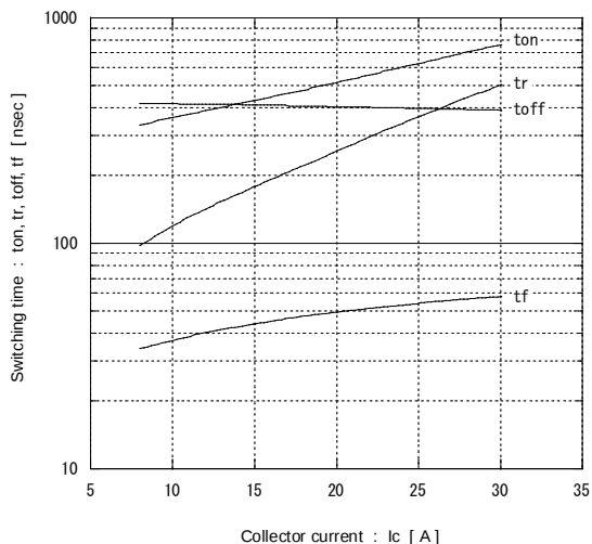
[ Inverter ] Switching time vs. Collector current (typ.) V_{CC}=300V , V_{GE}=+15V , R_g=270\Omega , T_j=25^\circ C
