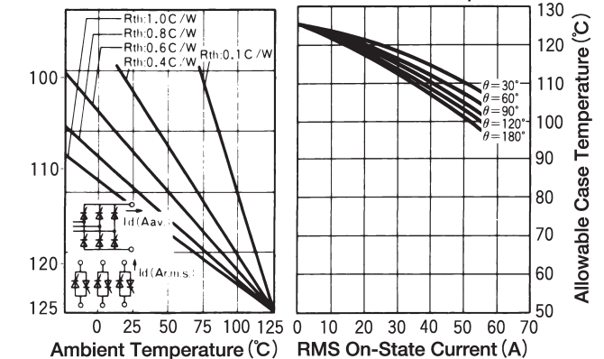
B6; Six pulse bridge connection W3; Three phase bidirectional connection
