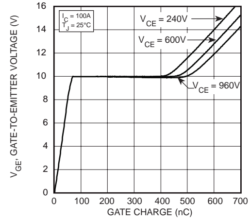
FIGURE 4, Gate charge
