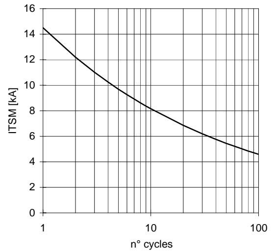
SURGE CHARACTERISTIC T_j = 125\text{ }^\circ\text{C}
