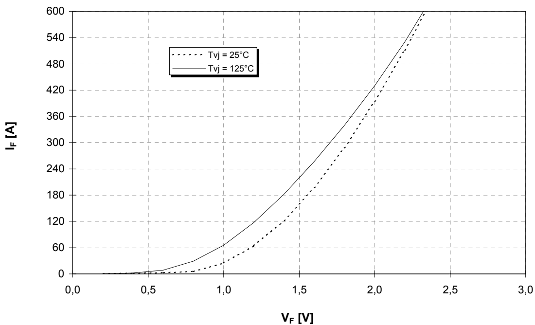
Forward characteristic of inverse diode (typical)
