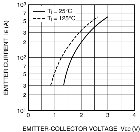
FREE-WHEEL DIODE FORWARD CHARACTERISTICS
