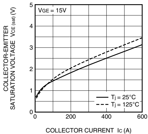
COLLECTOR-EMITTER SATURATION VOLTAGE CHARACTERISTICS
