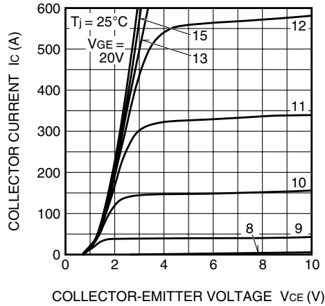
OUTPUT CHARACTERISTICS
