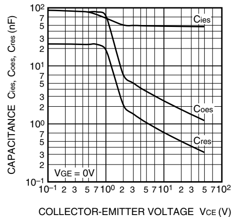
CAPACITANCE-VCE CHARACTERISTICS
