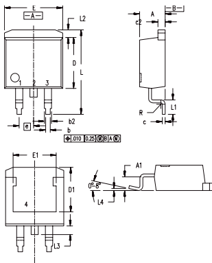
TO 263 AA
