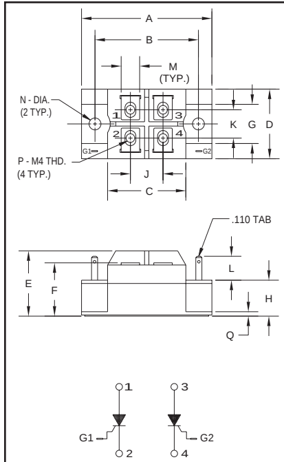
Outline Drawing
