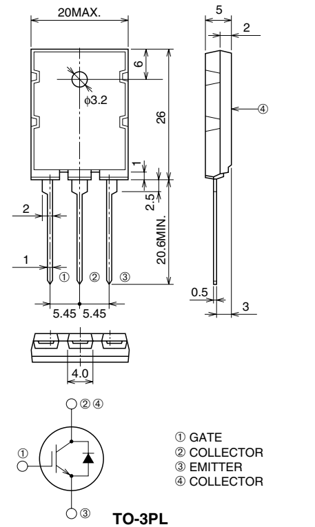
OUTLINE DRAWING
