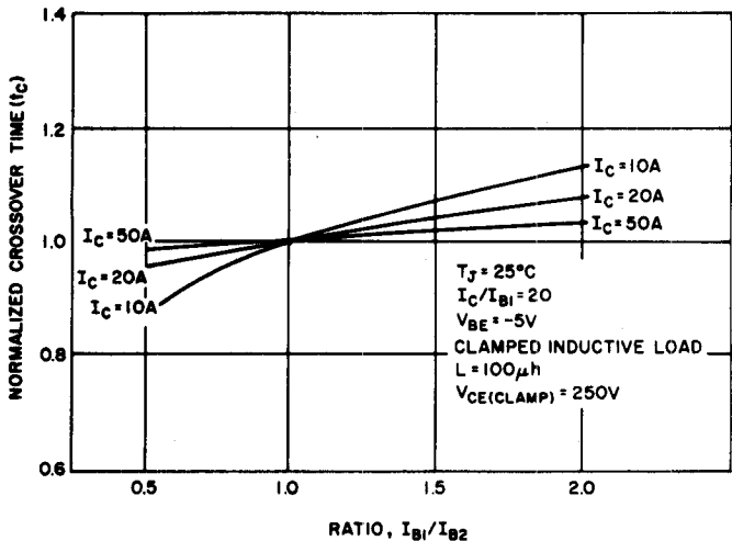
FIGURE 21. CROSSOVER TIME VARIATION WITH I_{B2} (D66DV ONLY)
