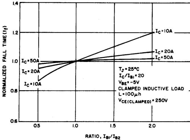
FIGURE 19. FALL TIME VARIATION WITH I_{B2} (D66DV ONLY)
