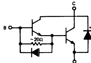
DEVICE CIRCUIT
